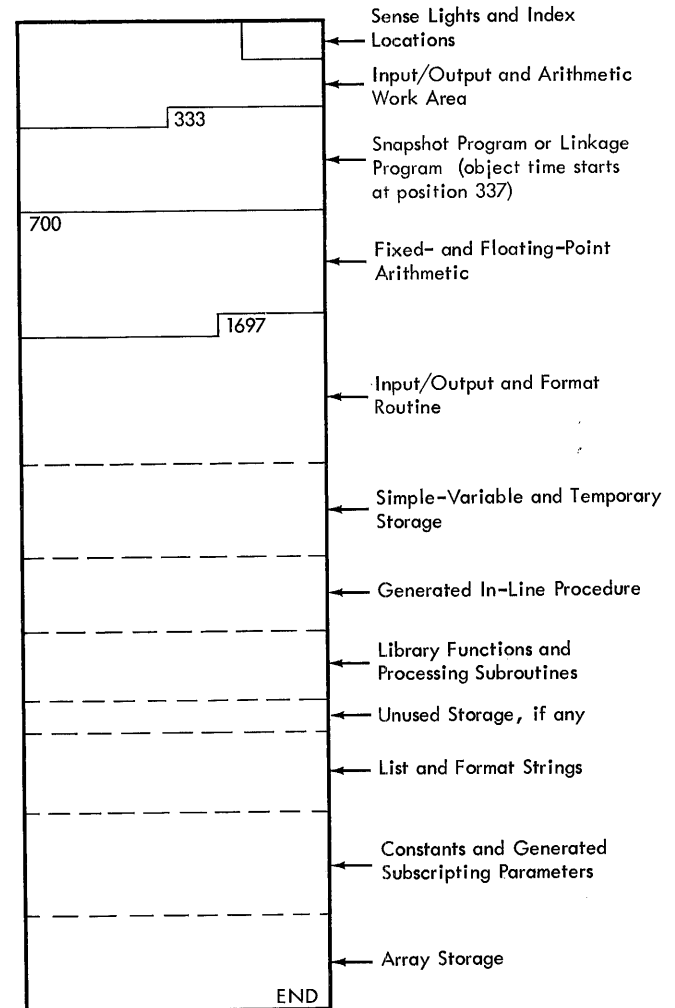
Figure 7. Object Program Storage Allocations
